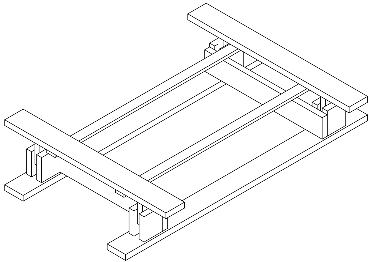
Boat Lift 3D Isometric View Scale: 1" = 1'-0"
