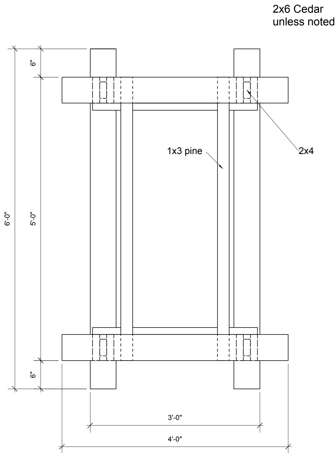
Boat Lift Plan View Scale: 1" = 1'-0"
